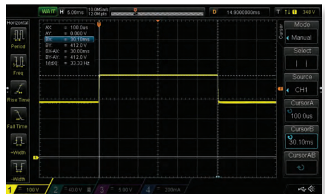
Figure 18: DO160G_AFX_16.6.1.4c_catZ_270V_Normal_Surge
