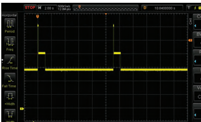
Figure 17: DO160G_AFX_16.6.2.4d_catB_28V_Abnormal_Surges
