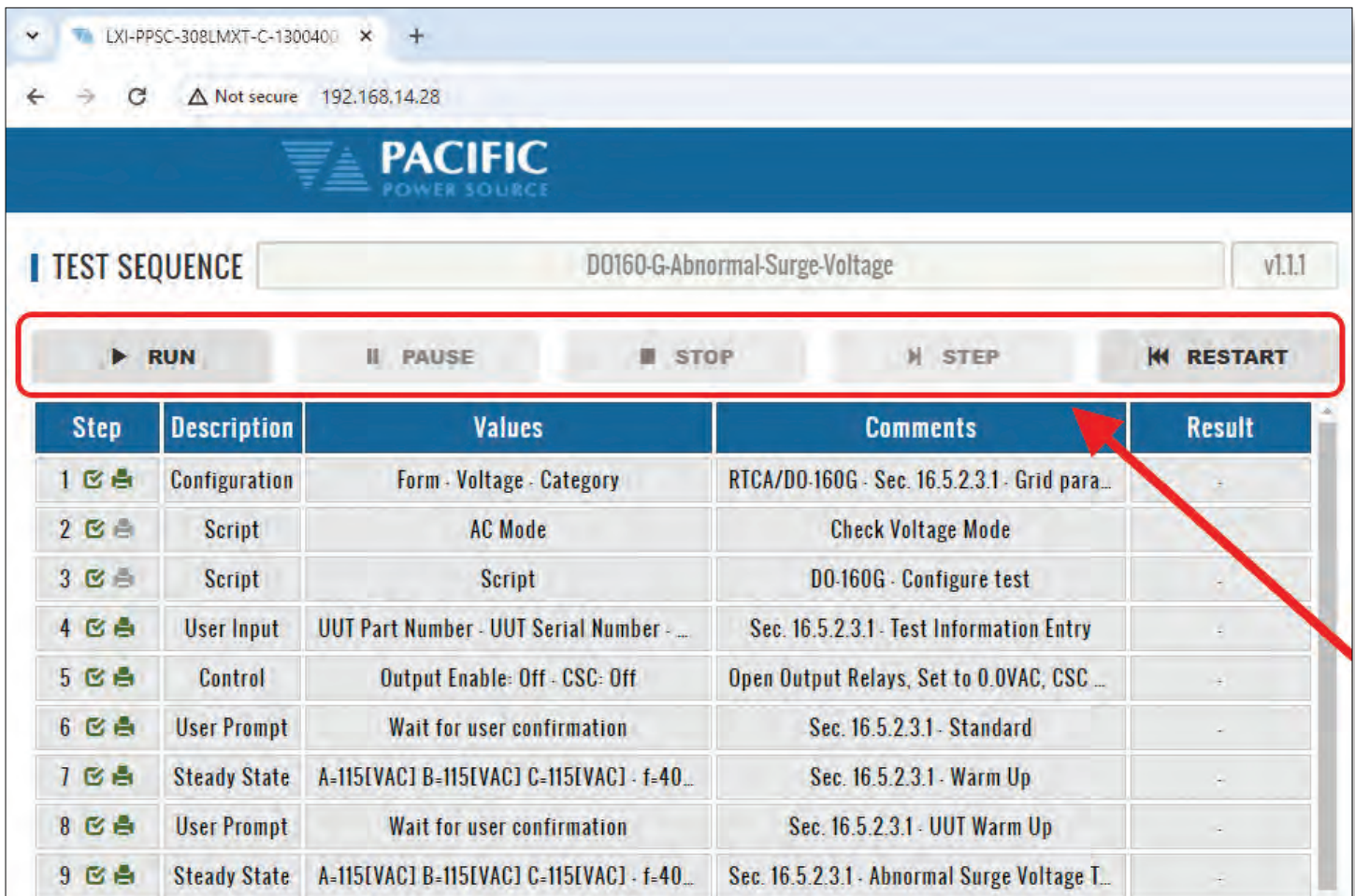
Figure 19: SmartSource Suite Web Browser User Execution Controls
