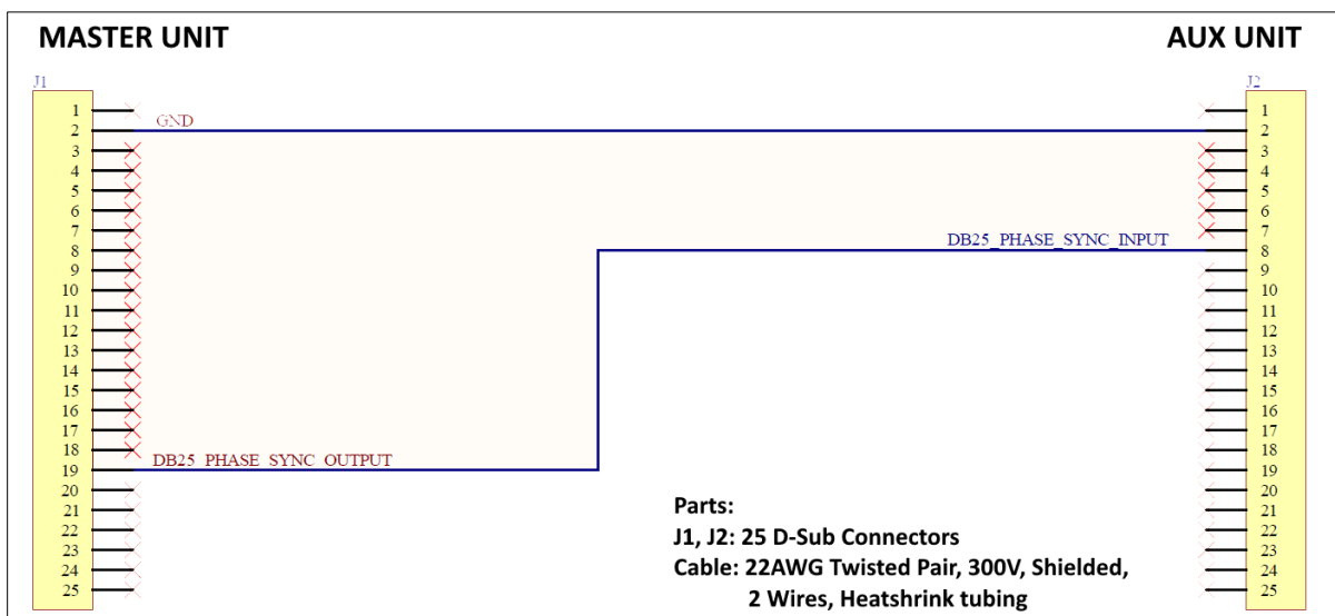
Figure 5: Sync Cable Assy Schematic
