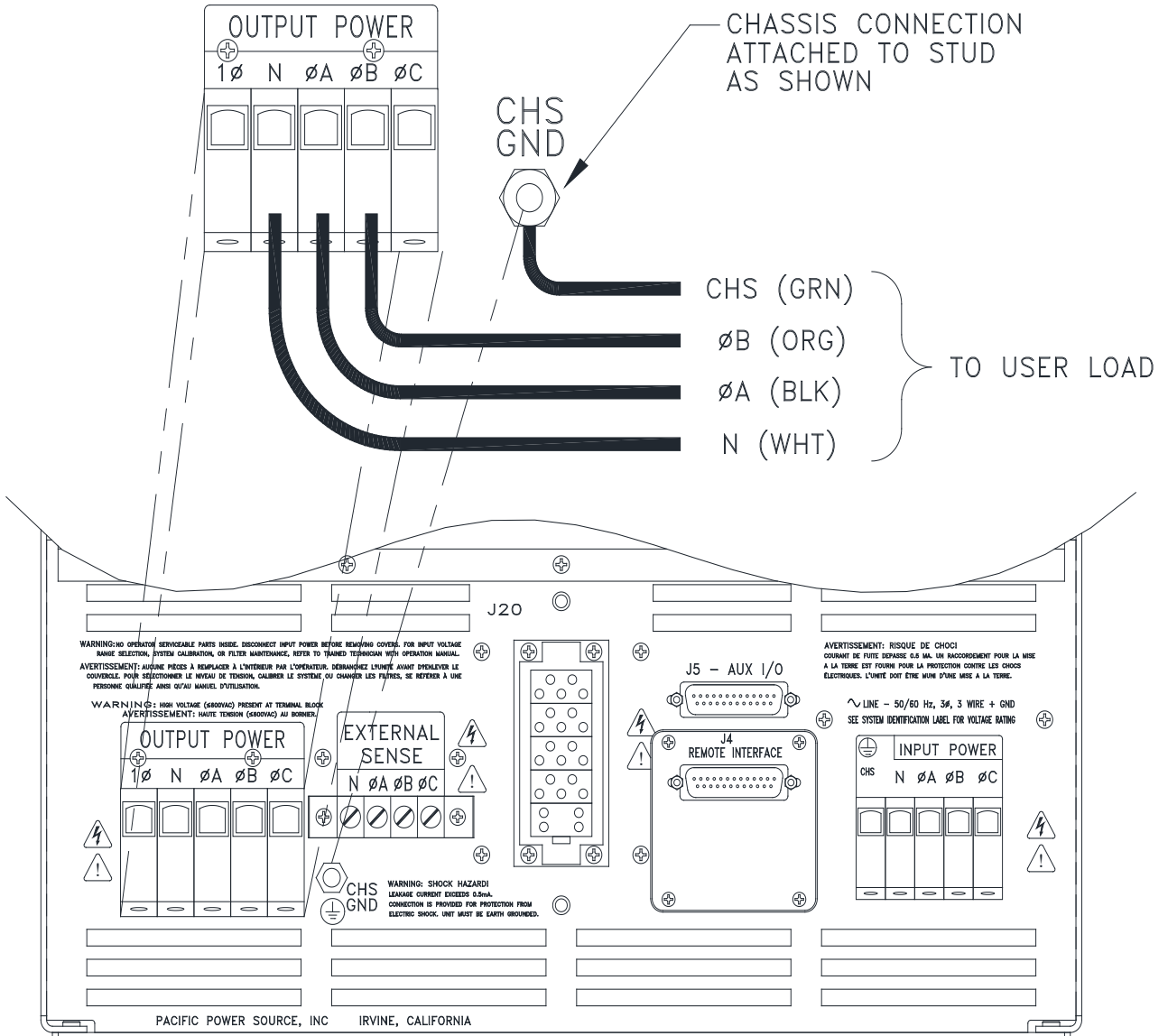
MODELS 390 & 3120-ASX REAR VIEW
