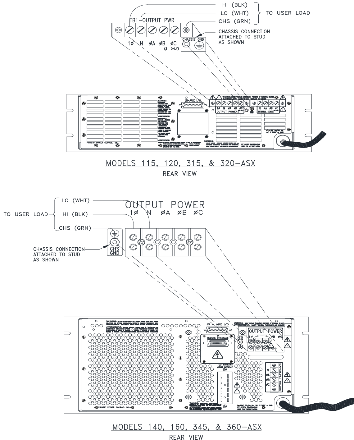
FIGURE 3.4.1.1 MODELS 115, 120, 140, 160, 315, 320, 345 & 360-ASX SINGLE PHASE OUTPUT CONNECTION
