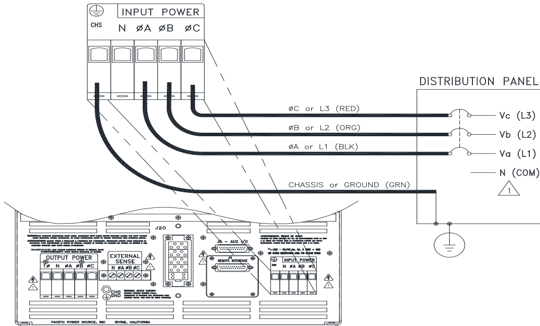
REAR VIEW
