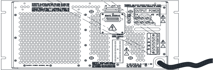
MODELS 140, 160, 345, & 360-ASX REAR VIEW
