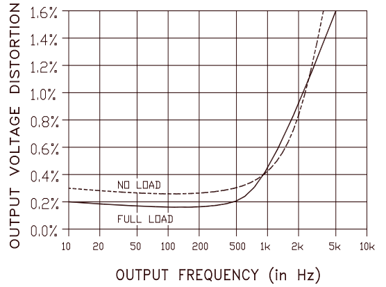
TYPICAL OUTPUT DISTORTION
