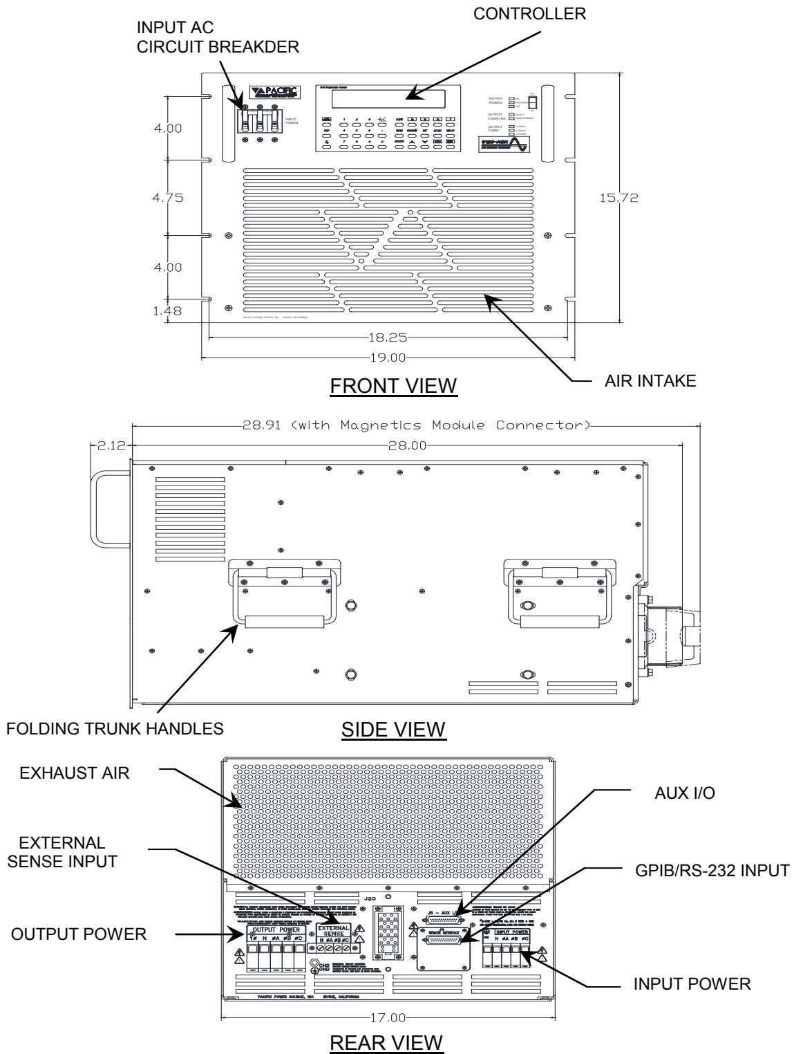
FIGURE 2.2.3 OUTLINE DRAWING, MODELS 390-ASX & 3120-ASX
