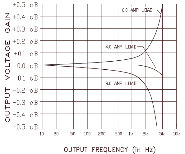
FREQUENCY RESPONSE
