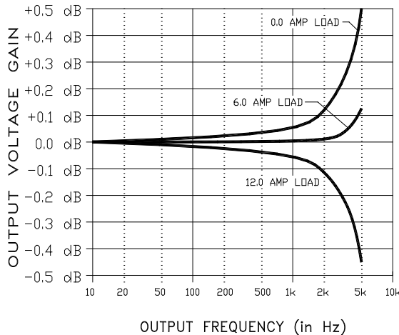
FIGURE 2.1.2 (A) MODEL 115-ASX OUTPUT RATING CURVES
