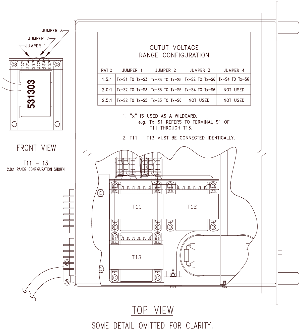
FIGURE 3.2.3 MODEL 315-ASX OUTPUT VOLTAGE RANGE CONFIGURATION (CUSTOM CONFIGURATION: SEE FACTORY FOR DETAILS)
