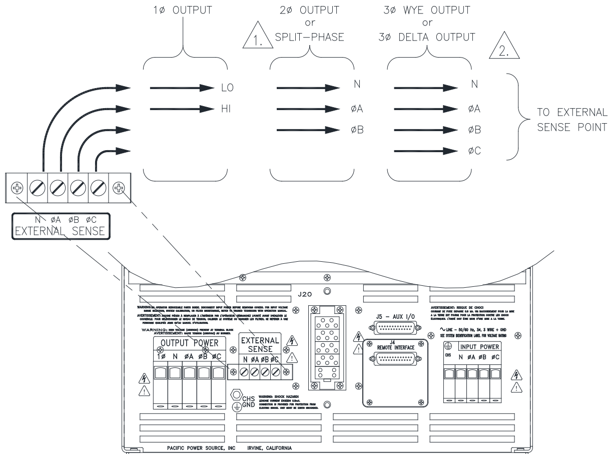
MODELS 390 & 3120-ASX REAR VIEW
