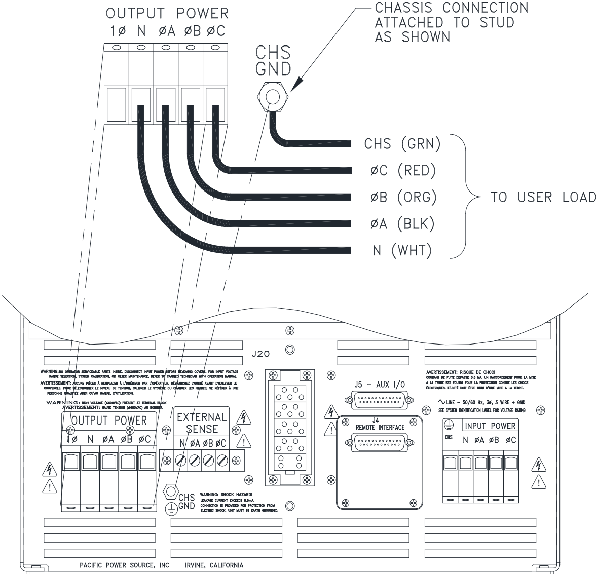
MODELS 390 & 3120-ASX REAR VIEW
