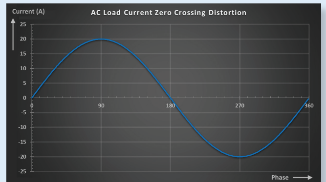
Figure 2: Regenerative AC Load Current
